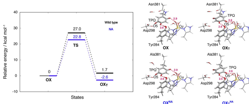
Fig. 8 Relative energies and related conformations for TPQ rotation in the oxidized form. Results for the WT and the N381A mutant are shown in black and blue, respectively. Most relevant distances between the heavy atoms are explicitly indicated.
