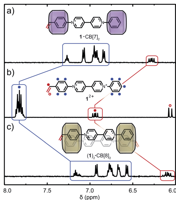
Fig. 2 Supramolecular complexation of 1 2+ and CB[ n ]. 1 H NMR spectra of 1 2+ at (a) \chi_{\text{CB}[7]} = 2 , (b) \chi_{\text{CB}[n]} = 0 and (c) \chi_{\text{CB}[8]} = 1 in D 2 O. Cl − counter-ions are omitted for clarity.
