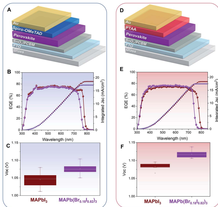
Fig. 5 \text{MAPbI}_3 and \text{MAPb}(\text{Br}_{0.18}\text{I}_{0.82})_3 perovskite solar cells (PSCs) (A) schematic of n-i-p PSCs with Spiro-OMeTAD as HMT, (B) EQE, (C) V_{oc} for \text{MAPbI}_3 and \text{MAPb}(\text{Br}_{0.18}\text{I}_{0.82})_3 . (D) Schematic of n-i-p PSCs with PTAA as HMT, (E) EQE, (F) V_{oc} for \text{MAPbI}_3 and \text{MAPb}(\text{Br}_{0.18}\text{I}_{0.82})_3 .
