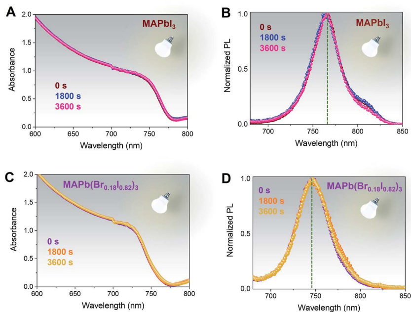
Fig. 4 \text{MAPbI}_3 and \text{MAPb}(\text{Br}_{0.18}\text{I}_{0.82})_3 light stability. UV-vis absorbance and photoluminescence spectra under continuous 1 sun illumination for over 3600 s for (A and B) \text{MAPbI}_3 and (C and D) \text{MAPb}(\text{Br}_{0.18}\text{I}_{0.82})_3 .
