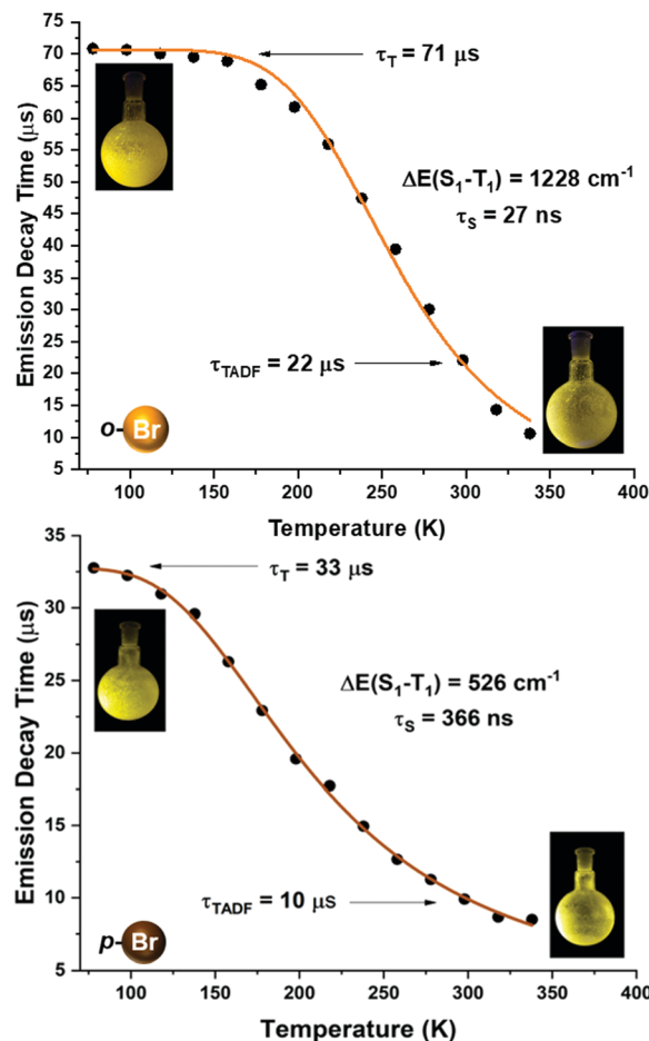
Fig. 7 Emission decay times of [\text{Au}(\text{o-C}_6\text{BrF}_4)(\text{dppBz})] ( 2 ) (top) and [\text{Au}(\text{p-C}_6\text{BrF}_4)(\text{dppBz})] ( 3 ) (bottom) versus temperature. The solid lines represent a fit of eqn (1) to the experimental data.
