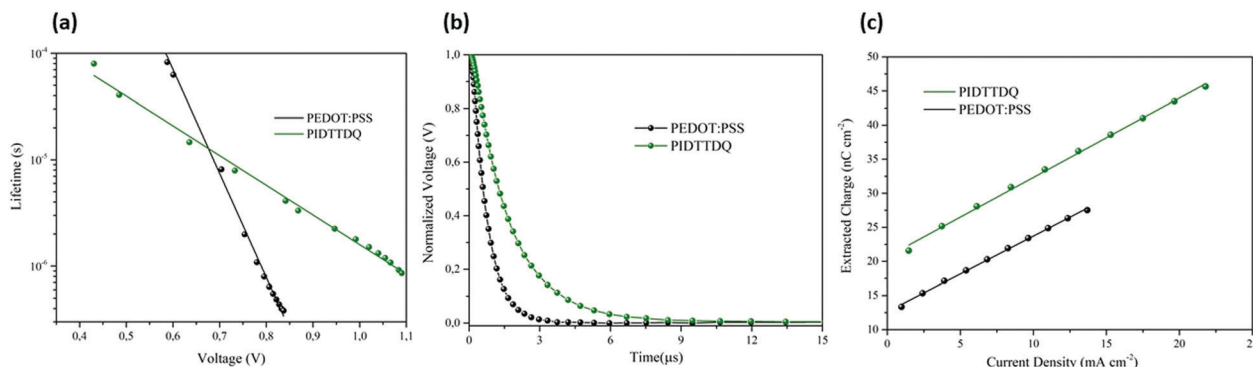
Fig. 5 (a) Lifetime obtained from TPV measurement as a function of voltage. (b) Normalized transient photovoltage decays under the same illumination for PIDTTDQ and reference device. (c) extracted charge density from TPC measurement as a function of current Density.
