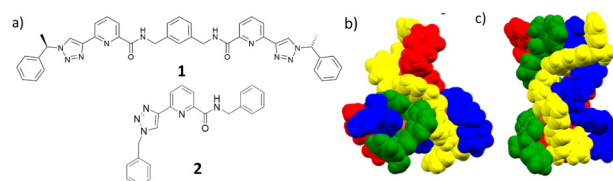
Fig. 1 (a) The chiral bis-tridentate (1,2,3-triazol-4-yl)-picolinamide (tzpa) ligand 1 used in the current study, and the ‘half’ ligand 2 , which was formed as a model ligand. The solid state structures of the tetranuclear [2 × 2] square grids formed from 1 in our previous study using: (b) Cu(NO 3 ) 2 · 3 H 2 O and (c) [Cu(MeCN) 4 ](PF 6 ), respectively. 26
