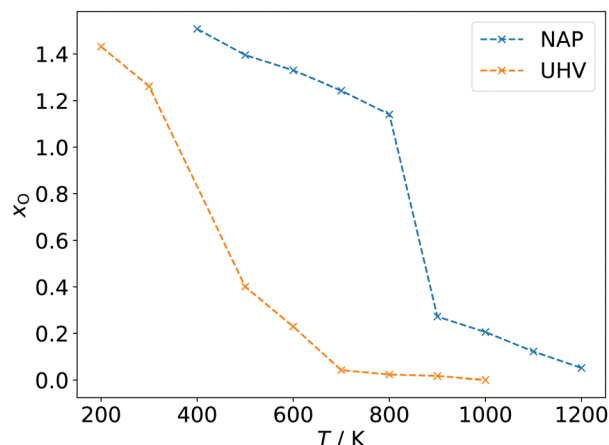
Fig. 11 Adsorption isobars for a 3 nm octahedral Pt particles oxidized at UHV ( p_O = 10^{-10} mbar) and NAP ( p_O = 1 mbar) conditions and 200–1200 K temperature. The degree of oxidation is quantified as the quotient between oxygen and platinum atoms in the system ( x_O = N_O/N_{Pt} ). Adapted from Kirchhoff et al. 26
