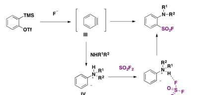
Scheme 7 Proposed reaction mechanism.
