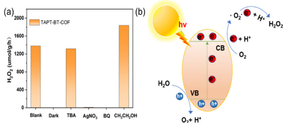
Fig. 6 Mechanism studies. (a) Photocatalytic \text{H}_2\text{O}_2 production of TAPT-BT-COF under different conditions. (b) Schematic diagram of the catalytic reaction mechanism.
