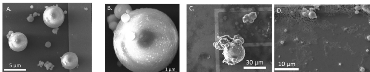
Fig. 1 SEM images of: A) fly ash sample PRB #1 showing spherical particles of varying sizes; B) a magnified view of PRB #1 showing multiple sized particles clustered together, including <1\text{ }\mu\text{m} particles attached to a 4\text{ }\mu\text{m} particle; C) fly ash App #1; D) fly ash App #2.
