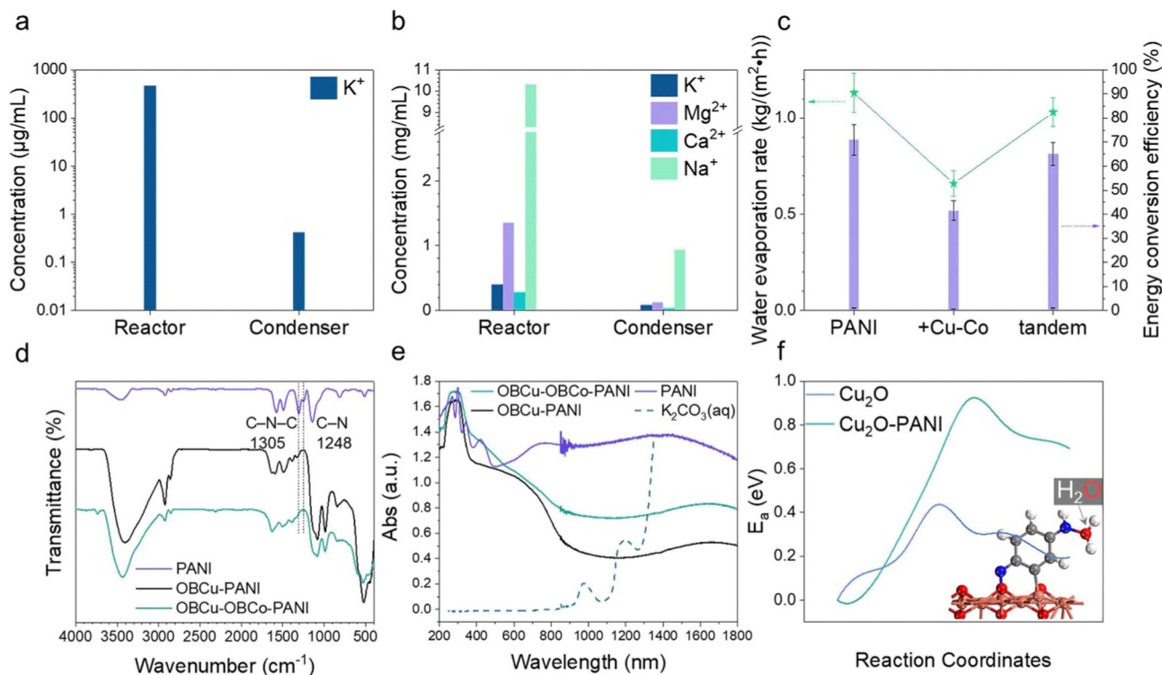
Fig. 5 (a) The ion concentration after water purification ( \text{K}_2\text{CO}_3(\text{aq.}) ) in the reactor and condenser. (b) The ion concentrations after seawater desalination in the reactor and condenser. (c) Water evaporation rate and corresponding energy conversion efficiency of PANI, OBCu-OBCo-PANI (+Cu-Co), and the tandem structure, with PANI beneath and OBCu-OBCo-PANI on top receiving the light first, half-thickness (tandem). (d) FTIR spectra of PANI, OBCu-PANI, and OBCu-OBCo-PANI. (e) UV-vis spectra of PANI, OBCu-PANI, OBCu-OBCo-PANI, and potassium carbonate solution. (f) The activation energy diagram calculation by NEB for the transfer of \text{H}_2\text{O} molecules from the solution to the catalytic surface.
