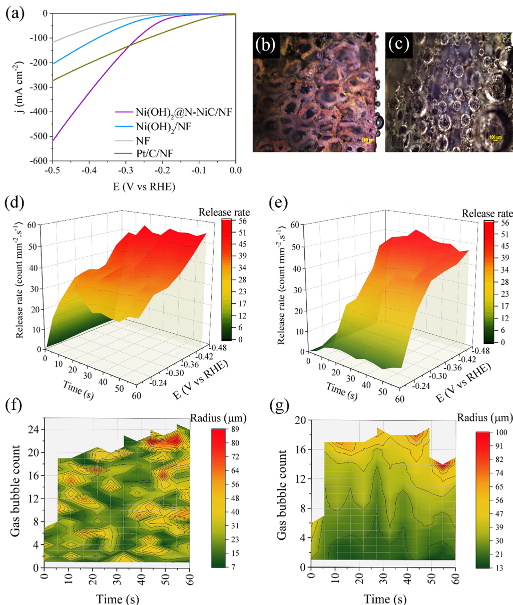
Fig. 2 (a) HER polarization curves. Optical images of gas bubbles over (b) \text{Ni}(\text{OH})_2\text{@N-NiC/NF} and (c) \text{Ni}(\text{OH})_2\text{/NF} at 0.245 V vs. RHE. Operando optical microscopy: 3D surface plots of (d) \text{Ni}(\text{OH})_2\text{@N-NiC/NF} and (e) \text{Ni}(\text{OH})_2\text{/NF} . Contour plots at 0.445 V vs. RHE for (f) \text{Ni}(\text{OH})_2\text{@N-NiC/NF} and (g) \text{Ni}(\text{OH})_2\text{/NF} .
