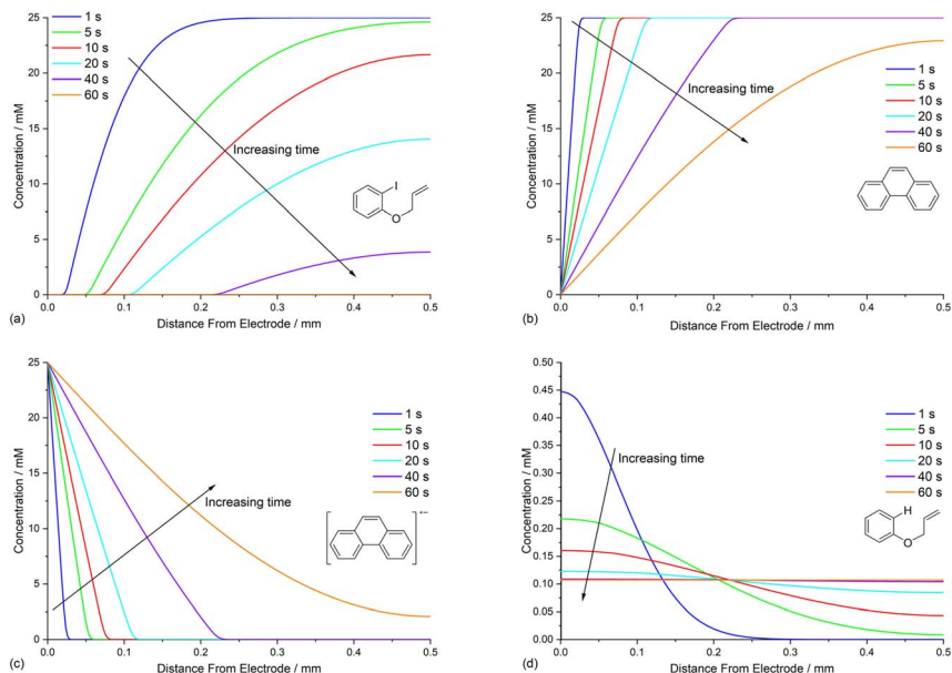
Fig. 3 Time dependent concentration profiles for electrolysis of Arl 1 in the presence of phenanthrene (1 equiv.) showing: (a) Arl 1. (b) Phenanthrene (M). (c) Phenanthrene radical anion (M •- ). (d) Hydrogenolysis product 3. Starting concentration of Arl 1 is 0.025 M. Electrolysis time = 0 to 60 s under constant potential of -2.8 V vs. SCE.
