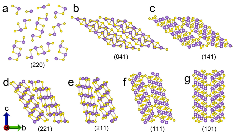
Fig. 16 Schematic of the (\text{Sb}_4\text{S}_6)_n ribbons with different crystal planes ( \text{Sb}^{3+} = purple dots and \text{S}^{2+} = yellow dots). Adapted with permission from ref. 1 Copyright 2022, Elsevier Ltd.
