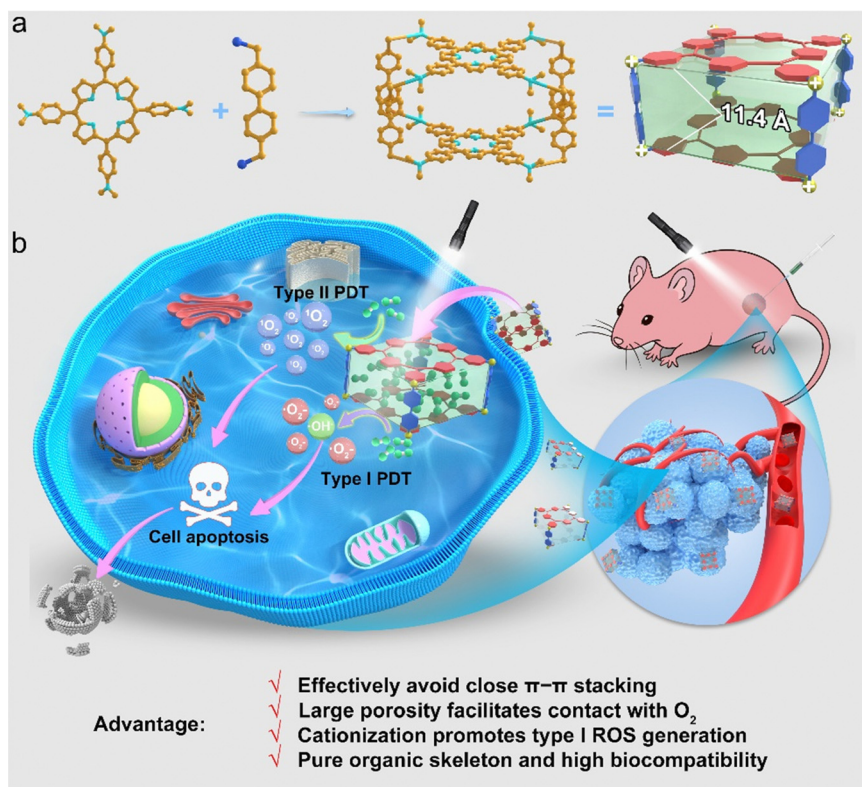
Scheme 1 (a) Schematic of the synthesis of the Py-Cage; (b) schematic of the working mechanism of the Py-Cage: the Py-Cage enhances the generation of type I ( \text{OH}^{\cdot} and \text{O}_2^{\cdot-} ) and type II ( \text{O}_2 ) ROS under white light irradiation to induce cell apoptosis and death for PDT applications.
