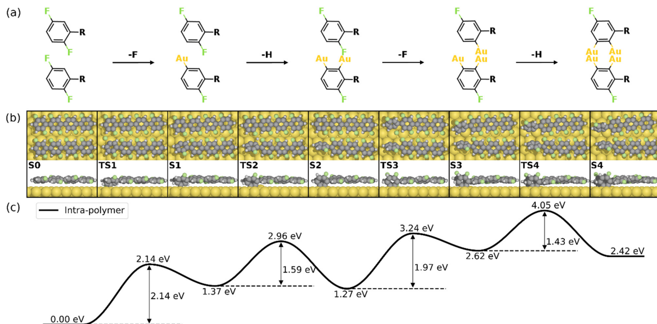
Fig. 3 Reaction mechanism of the first four steps of the HF zipping reactions ( S0–S4 ). (a) Valence bond structures for each intermediate state. (b) The reaction pathway and (c) the corresponding energy profile. Definition of energies is given in eqn (S3) (see ESI†). The C, H, F, and Au atoms are represented by the gray, white, green, and yellow circles, respectively.
