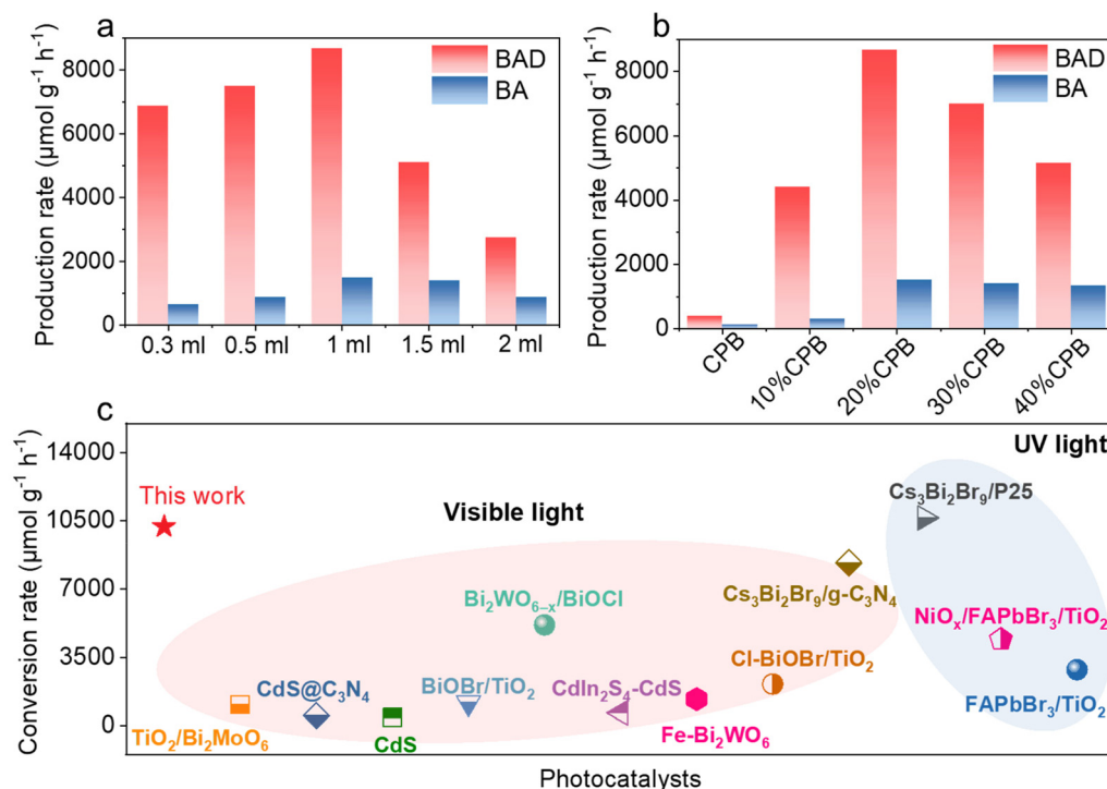
Fig. 5 (a) Photocatalytic oxidation of toluene with different toluene amounts in acetonitrile solvent over 20%CPB/ \text{TiO}_2 . The total volume is 3 mL. (b) Photocatalytic oxidation of toluene over blank \text{TiO}_2 , CPB/ \text{TiO}_2 composite and blank \text{CsPbBr}_3 . (c) Performance comparison with reported photocatalysts for UV and visible-light-driven selective oxidation of toluene.
