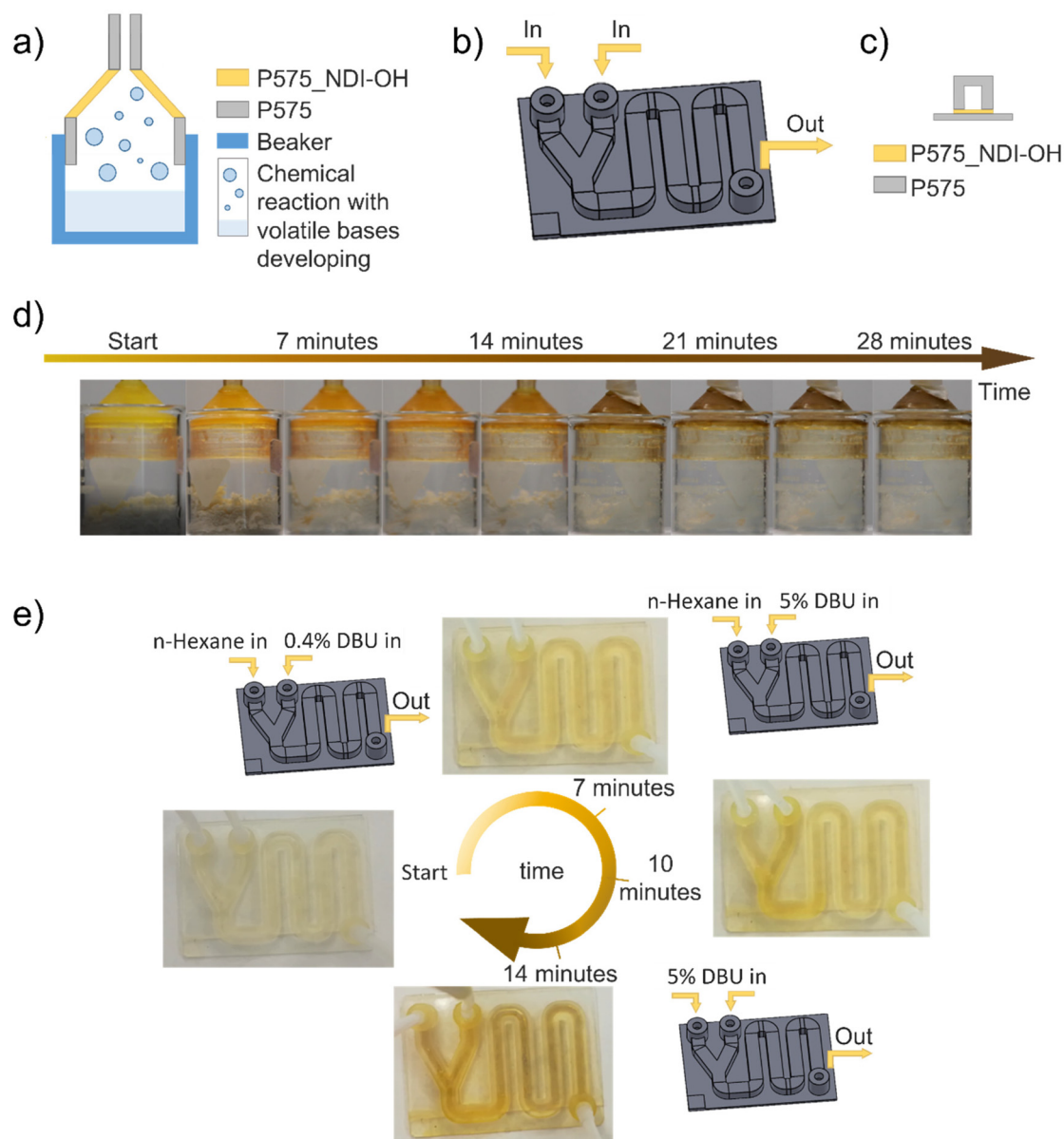
Fig. 5 (a) Schematic representation of the smart lid's composition and application; (b) schematic representation of the fluidic application; (c) schematic representation of the generated vapor; (d) smart lid application to monitor the evolution of the reaction reported in formula (1), by sensing the generated vapor; (e) demonstration of the fluidic application by feeding solution with different DBU concentration. Pictures show the final color reached at the end of the tests, drawings are schematic representations of the test feeding solutions.
