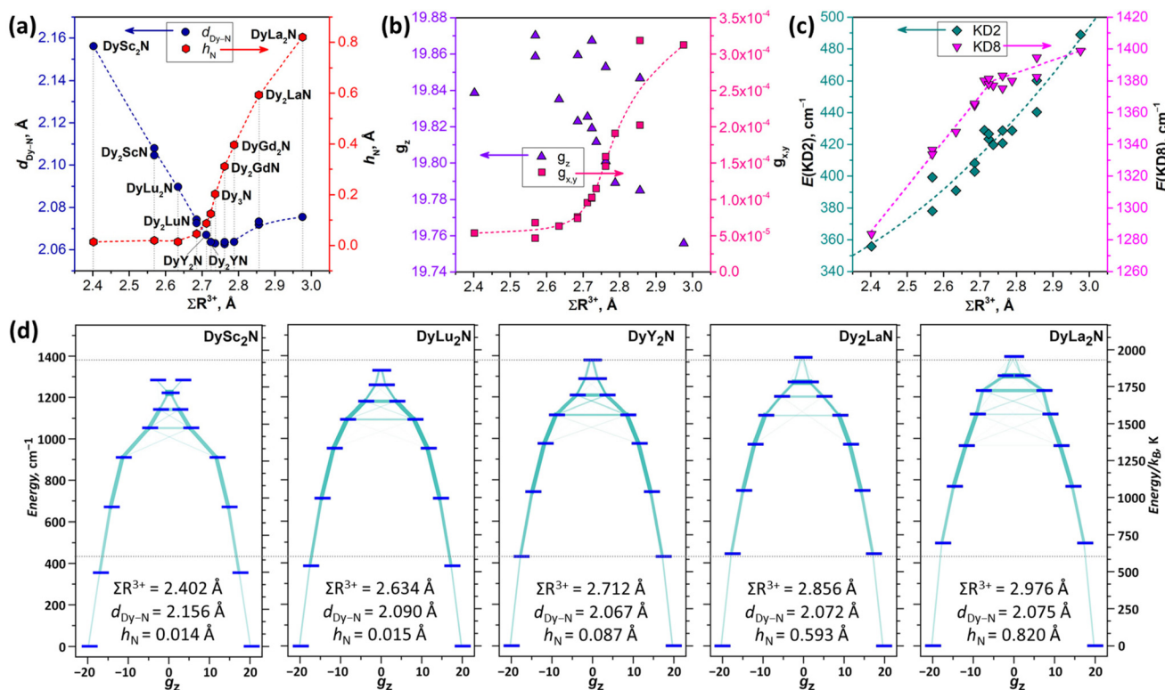
Fig. 5 (a) Dy–N bond lengths ( d_{\text{Dy-N}} ) and M_3\text{N} pyramid height (elevation of N above the plane of metal atoms, h_N ) in DFT-optimized \text{DyM}_2\text{N}@C_{80} and \text{Dy}_2\text{MN}@C_{80} molecules ( M = \text{Sc}, \text{Lu}, \text{Y}, \text{La}, \text{Gd} ) plotted versus the sum of Shannon's ionic radii of metals in the M_3\text{N} cluster ( \Sigma R^{3+} ). (b) Components of the pseudospin g -tensor, g_z and g_{x,y} (root mean square of g_x and g_y ) for the \text{Dy}^{3+} ground state Kramers doublet (KD1) in the same set of molecules. (c) The energy of the first excited KD (KD2) and the total ligand-field splitting (KD8) in the same set of molecules. Dashed lines in (a) and (b) are a spline interpolation added to guide the eye; in (c), the dashed line for E(\text{KD2}) is a quadratic fit. (d) \text{Dy}^{3+} ligand-field splitting with transition probabilities in selected M_3\text{N}@C_{80} molecules along with their \Sigma R^{3+} , d_{\text{Dy-N}} , and h_N parameters; dotted lines are guides to the eye and mark the KD2 and KD8 energies in \text{Dy}_2\text{N}@C_{80} . Ligand-field splitting and pseudospin g -tensor parameters used in (b–d) are computed ab initio at the CASSCF/RASSI-SO level using DFT-optimized molecular structures.
