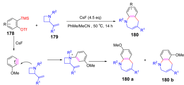
Scheme 25 2-Vinylazetidines with benzene of the [6 + 2] cycloaddition reaction.
