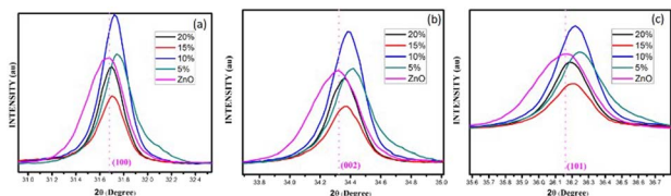
Fig. 4 The shifts in peak position in the X-ray diffraction angles corresponding to (a) (100), (b) (002) and (c) (101) planes for as-synthesized pure ZnO powder and \text{AlCl}_3 @ZnO powders corresponding to wt% loadings of 5%, 10%, 15%, and 20%.
