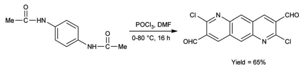
Scheme 49 Synthesis of 2,7-dichloropyrido[2,3-g]quinoline-3,8-dicarbaldehyde.
