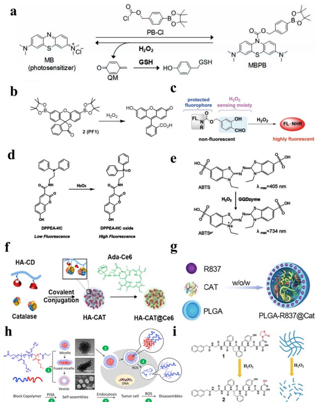
Fig. 2 (a) A schematic diagram illustrating of MBPBP to deliver methylene blue. Reproduced from ref. 47 copyright 2019, Elsevier Ltd. (b) A schematic diagram illustrating \text{H}_2\text{O}_2 -related fluorescent conversion of PF1. Reproduced from ref. 49 copyright 2004, American Chemical Society. (c) Schematic of a tandem Payne/Dakin reaction. Reproduced from ref. 54 copyright 2018, Wiley-VCH Verlag GmbH & Co. KGaA, Weinheim. (d) A schematic diagram illustrating the fluorescence intensity of DPPEA-HC enhanced. Reproduced from ref. 56 copyright 2004, Elsevier Ltd. (e) A schematic diagram illustrating the conversion of ABTS in the presence of \text{H}_2\text{O}_2 . Reproduced from ref. 57 copyright 2019, American Chemical Society. (f) The preparation process of HA-CAT@Ce6 by the conjugation of HA with CAT. Reproduced from ref. 63 copyright 2019, American Chemical Society. (g) Schematic of PLGA to encapsulate CAT. Reproduced from ref. 64 copyright 2019, WILEY-VCH Verlag GmbH & Co. KGaA, Weinheim. (h) Schematic of the evolution of particle size and morphology of \text{H}_2\text{O}_2 -sensitive block copolymer NPs. Reproduced from ref. 65 copyright 2022, American Chemical Society. (i) Schematic of releasing drugs via \text{H}_2\text{O}_2 -responsive hydrogels. Reproduced under terms of the CC-BY license. 71 Copyright 2017, Chunhua Ren, published by RSC Advances.
