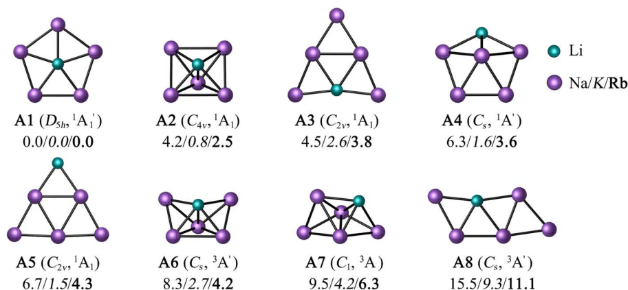
Fig. 1 PBE0-D3/def2-QZVPP geometries of the low-lying energy isomers of \text{LiM}_5 ( M = \text{Na/K/Rb} ). Relative energies in kcal mol -1 were computed at the CCSD(T)/def2-QZVPP//PBE0-D3/def2-QZVPP level, including the zero-point energy computed at the DFT level. Point groups and spectroscopic states are given in parentheses.
