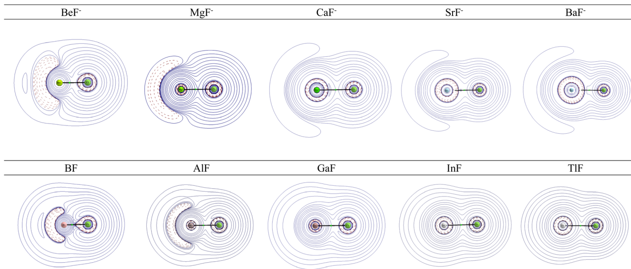
Fig. 2 Laplacian distribution \nabla^2 \rho(r) of \text{AeF}^- ( \text{Ae} = \text{Be}-\text{Ba} ) and \text{EF} ( \text{E} = \text{B}-\text{Tl} ) at the CCSD(T)/def2-TZVPP level. Red lines indicate the areas of charge concentration ( \nabla^2 \rho(r) < 0 ), while blue lines show the areas of charge depletion ( \nabla^2 \rho(r) > 0 ). The solid lines connecting the atomic nuclei are the bond paths. Green dots are bond critical points.
