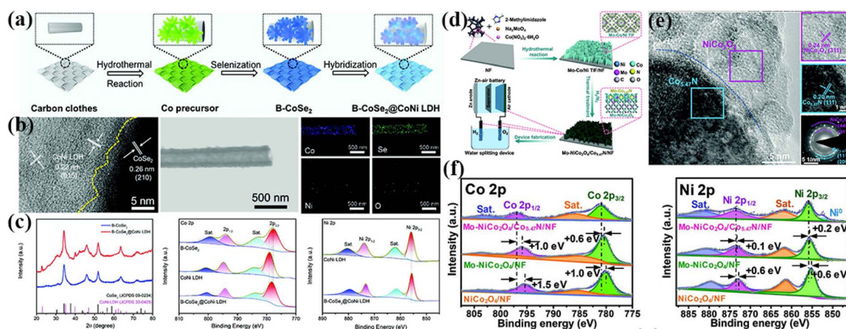
Fig. 7 (a) Schematic illustration of the synthetic process of B- \text{CoSe}_2@/\text{CoNi} LDH HNA. (b) HRTEM image of B- \text{CoSe}_2@/\text{CoNi} LDH HNA high-lighting the interface between \text{CoSe}_2 and CoNi LDH and elemental mapping images of B- \text{CoSe}_2@/\text{CoNi} LDH HNA. (c) XRD spectra and XPS patterns for B- \text{CoSe}_2 , CoNi LDH, and B- \text{CoSe}_2@/\text{CoNi} LDH HNA. Reproduced with permission from ref. 152, Copyright (2022) Wiley. (d) Schematic illustration of the synthetic process of Mo–NiCo 2 O 4 /Co 5.47 N/NF. (e) HRTEM images and SAED pattern of Mo–NiCo 2 O 4 /Co 5.47 N/NF. (f) XPS spectra of Mo–NiCo 2 O 4 /Co 5.47 N/NF, Mo–NiCo 2 O 4 /NF, and NiCo 2 O 4 /NF. Reproduced with permission from ref. 154, Copyright (2020) Wiley.
