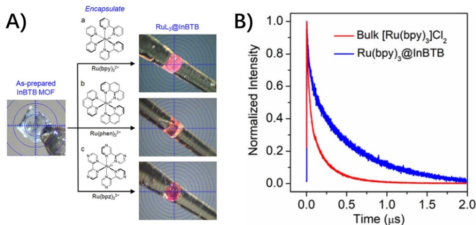
Fig. 7 (A) Photo images of the colorless as-prepared InBTB and the color change in \text{RuL}_3@ \text{InBTB} MOFs. (B) Normalized time-resolved photoluminescence decay curves obtained for bulk [\text{Ru}(\text{bpy})_3]\text{Cl}_2 and \text{Ru}(\text{bpy})_3@ \text{InBTB} upon excitation at 470 nm. Adapted from ref. 67 with permission from Wiley-VCH.
