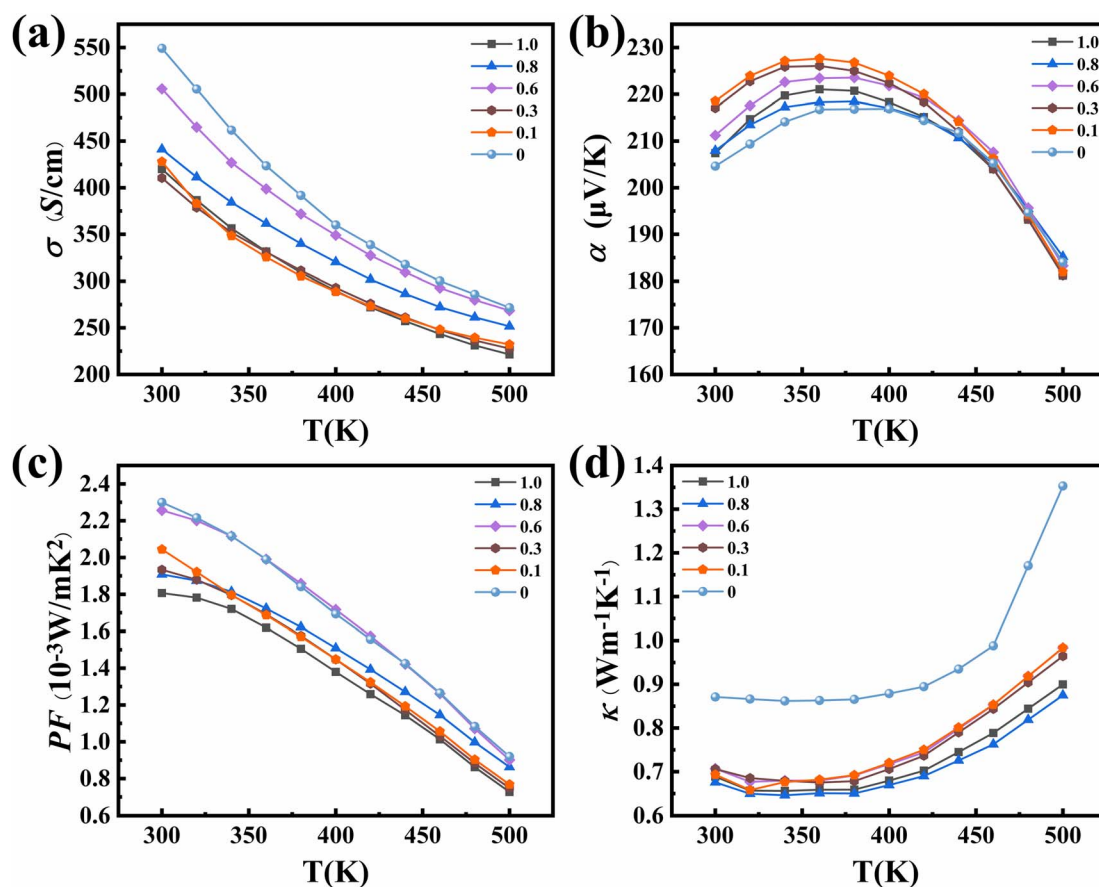
Fig. 5 (a) Electrical conductivity, (b) Seebeck coefficient, (c) power factor, and (d) thermal conductivity of \text{Bi}_{0.5}\text{Sb}_{1.5}\text{Te}_3/\text{x vol}\% SiC ( x = 0, 0.1, 0.3, 0.6, 0.8, 1.0 ) as a function of temperature.
