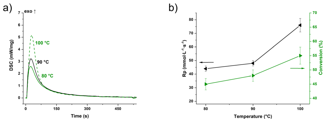
Fig. 2 (a) Photo-DSC of the PT-30 formulation at 80–100 °C, 2 \times 900 s, 320–500 nm, 60 mW cm -2 . (b) Temperature dependence of rate of polymerization ( R_p , black) and conversion of the cyanate ester groups (green).
