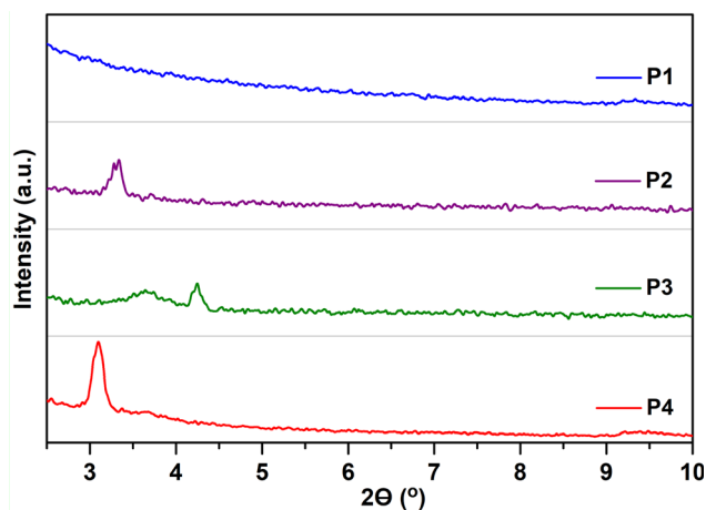
Fig. 8 GIXRD patterns of P1–P4 thin films prepared under optimal device performance conditions. An intensity spectral range from 0 to 350 a.u. was used for all polymers.
