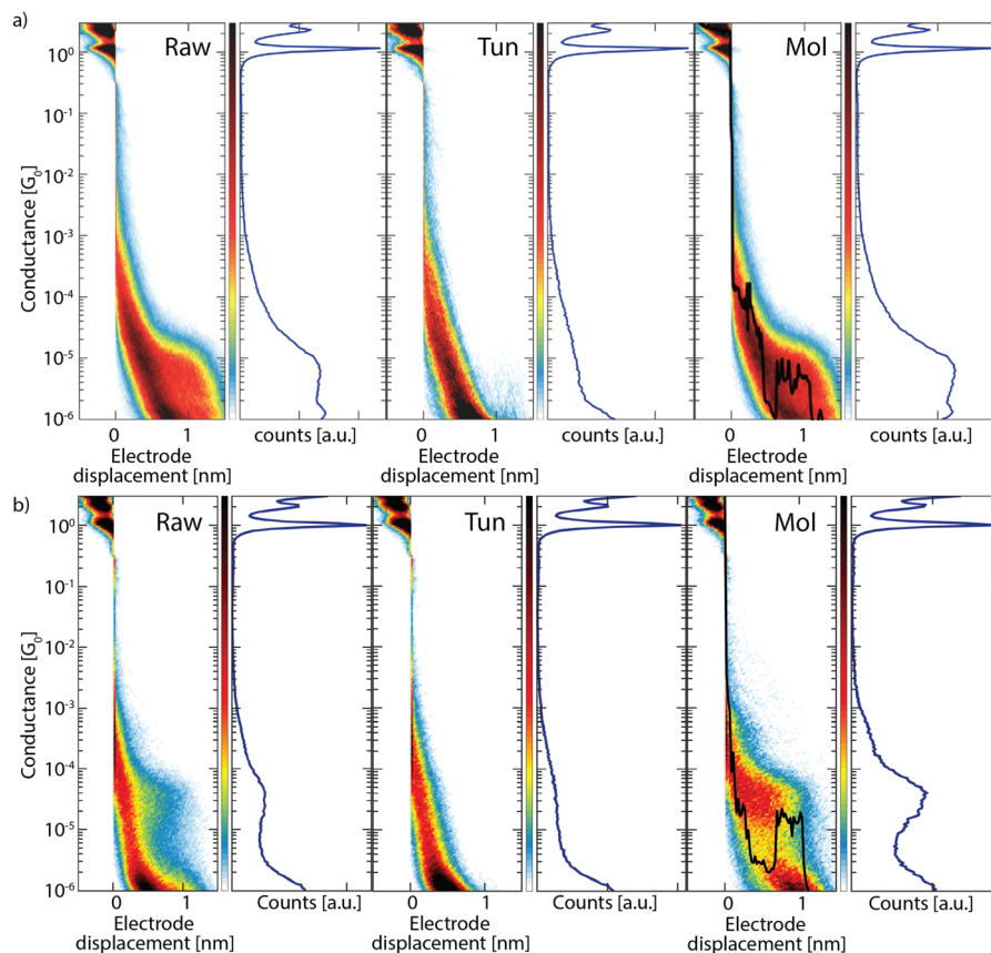
Fig. 4 Tunnelling separation performance of our trained network on unseen experimental measurement sets of breaking traces recorded for OPE3-Pyr (a) and OPE3- \text{NH}_2 (b), showing the histogram of the complete data set (left), and the histograms constructed from the separated tunnelling-only (middle) and remaining molecular traces on the right (right). The molecular classes for both molecules contain a single blue-colored example trace.
