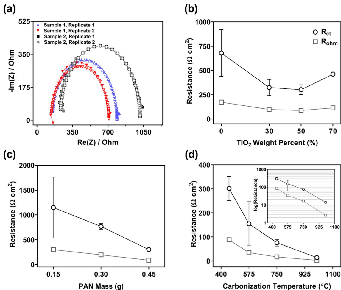
Fig. 4 (a) Typical Nyquist plots obtained from PEIS data ( \blacktriangle ) for 0.45 g PAN/50 wt% TiO 2 composites and corresponding fit ( \Delta ) by the Simple Randles circuit (see Fig. S5 † ). The data demonstrate consistency between replicates and batches. (b) Charge transfer resistance ( R_{ct} ) and ohmic resistance ( R_{ohm} ) for 0.45 g PAN/TiO 2 composites. Standard deviation for 70 wt% composite is small relative to scale. (c) R_{ct} for 50 wt% TiO 2 composites with varying PAN mass (0.15, 0.30, and 0.45 g). (d) R_{ct} and R_{ohm} for 0.45 g PAN/50 wt% TiO 2 electrodes carbonized at 450, 575, 750, and 1000 °C. PEIS parameters are listed in the ESI. †
