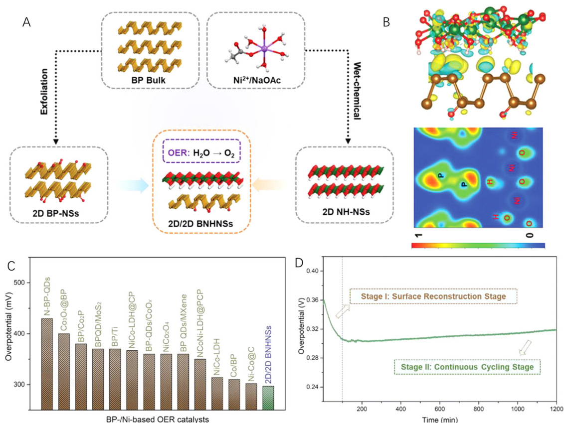
Fig. 6 (A) Schematic illustration of the synthesis of 2D–2D heterostructured nanosheets (BNHNSs) by coupling 2D \text{Ni}(\text{OH})_2 nanosheets (NH-NSs) and 2D black phosphorus (BP) nanosheets (BP-NSs). (B) The charge density difference and electron localization function maps of 2D–2D BNHNSs. (C) Comparison of the overpotentials with those of the reported electrocatalysts at 10 \text{ mA cm}^{-2} . (D) Time-dependent overpotential curve of the 2D–2D BNHNSs catalyst in KOH for 1200 min. Reproduced with permission from ref. 92, copyright Wiley.
