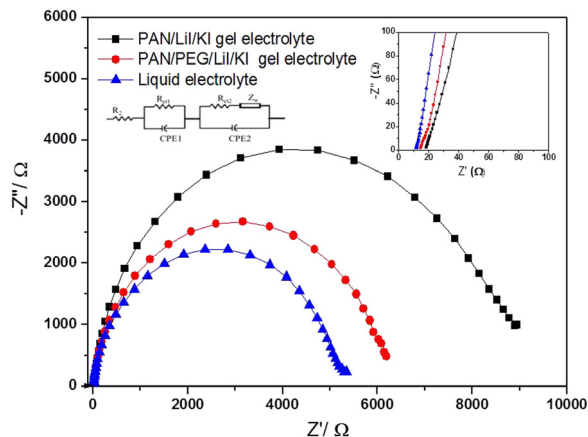
Fig. 6 The impedance spectra of the DSSC based on liquid electrolyte, PAN/LiI/KI and PAN/PEG/LiI/KI blend GPEs. The inset plot shows the contact resistance between the electrolyte and the Pt electrode interface.
