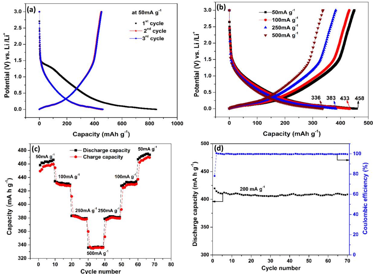
Fig. 5 Galvanostatic charge discharge profiles of CNTs on the Cu substrate. (a) First three charge–discharge cycles at 50 \text{ mA g}^{-1} . (b) Electrode subjected to various current densities from 50 – 500 \text{ mA g}^{-1} . (c) High-rate cycling performance. (d) Discharge capacity and coulombic efficiency vs. cycle number at the current density of 200 \text{ mA g}^{-1} .
