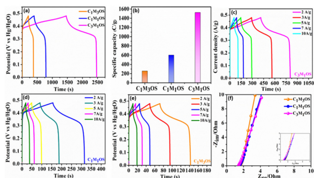
Fig. 5 Three-electrode electrochemical measurements: (a) and (b) GCD profiles and the corresponding specific capacity of the C_1M_3OS , C_1M_1OS , and C_3M_1OS electrodes at a current density of 1\text{ A g}^{-1} . GCD profiles at various current densities ( 2\text{--}10\text{ A g}^{-1} ) of (c) C_3M_1OS , (d) C_1M_1OS , and (e) C_1M_3OS . (f) Nyquist plots for the designed C_1M_3OS , C_1M_1OS , and C_3M_1OS electrodes.
