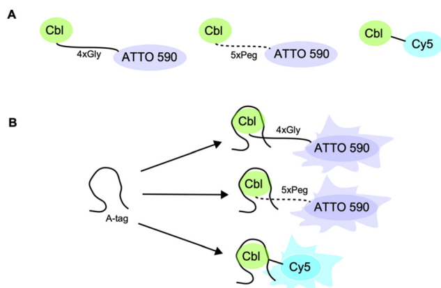
Fig. 1 Riboglow probes used in this study. (A) Representation of Riboglow Cbl-fluorophore probe variants evaluated in this study and (B) representation of Riboglow probes binding to the RNA tag (called the A-tag throughout this study) leading to a change in fluorescence lifetime.
