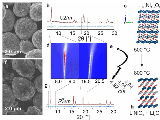
Fig. 1 (a) SEM image, (b) XRD pattern including refinement plot, and (c) illustration of the crystal structure of \text{Li}_{1+x}\text{Ni}_{1-x}\text{O}_2 . (d) Zoomed-in view of the XRD raw data from an in situ heating experiment (from 500 to 800 °C) and (e) corresponding refined layering parameter c/a . (f) SEM image, (g) XRD pattern including refinement plot, and (h) illustration of the crystal structure of \text{LiNiO}_2 obtained by thermal decomposition of \text{Li}_{1.2}\text{Ni}_{0.8}\text{O}_2 at 750 °C.
