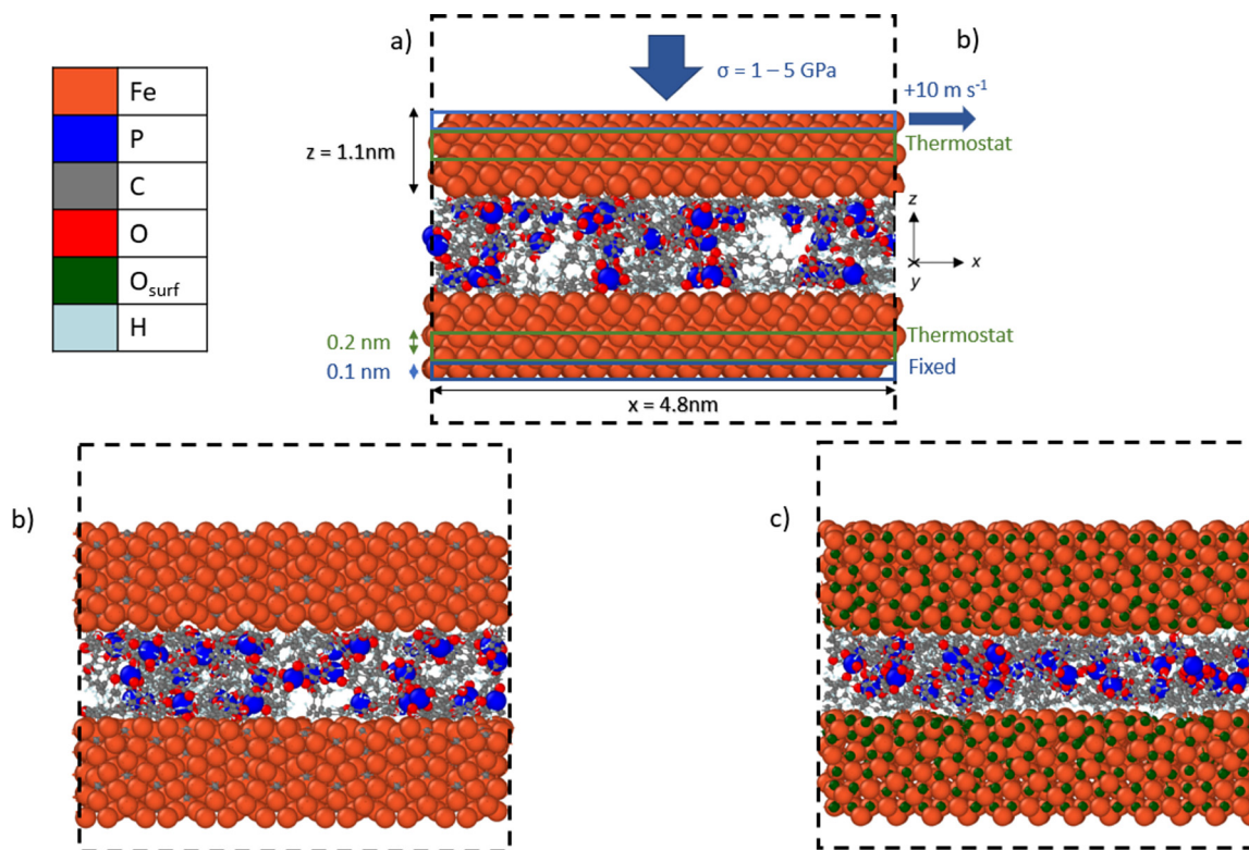
Fig. 2 Side-view snapshots showing the model systems with TCP molecules confined between (a) \alpha\text{-Fe}(110) , (b) \text{Fe}_3\text{C}(010) , and (c) \text{Fe}_3\text{O}_4(001) -SCV surfaces. Systems shown after minimisation and equilibration, but before heating, compression, and shear. Black dashed line shows the simulation box. Rendered using OVITO. 42
