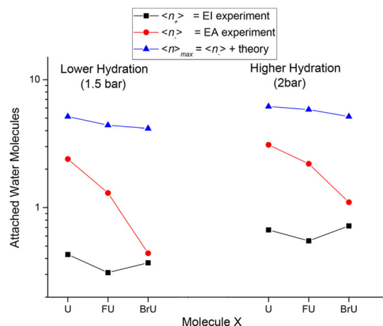
Fig. 4 The image from the work of Poštolka et al. showing that theory predicted increase in the energy transfer to solvent due to the electron affinity of the microhydrated halo uracils can reproduce well the fragmentation of their TNIs. For uracil (U), bromouracil (BrU) and fluorouracil (FU) shown on the x-axis the y-axis shows the detected mean size of ionic clusters upon electron attachment (red) and electron ionization (black). The blue points are mean values of neutral cluster sizes estimated based on electron affinities and under the assumption that all energy transferred to solvent leads to the evaporation of water molecules from the cluster. Reproduced from ref. 52 with permission from American Chemical Society, copyright 2017.
