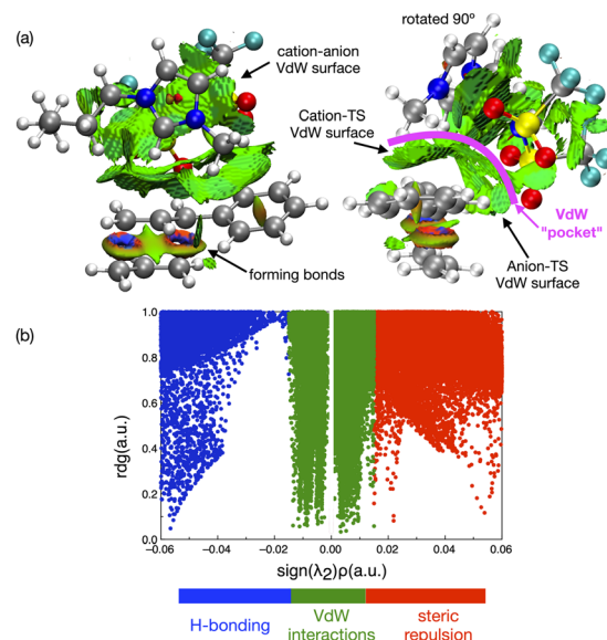
Fig. 12 (a) NCI plots of the interaction of the TS-IL [C 4 C 1 im][NTf 2 ] cluster from different directions (cation forward, and anion forward) showing substantial VdW interaction surfaces. (b) Graph of the reduced density gradient, against the density \rho(r) multiplied by the sign of the second eigenvalue from \nabla^2\rho(r) , \text{sign}(\lambda_2) .
