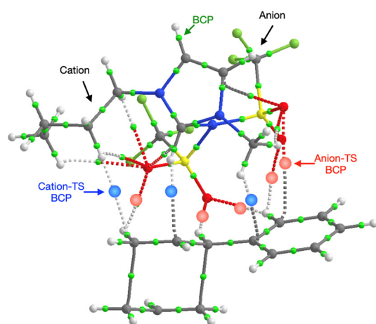
Fig. 11 AIM plot of BCPs linking the ion-pair of [C 4 C 1 im][NTf 2 ] with the TS in TS-IL.
