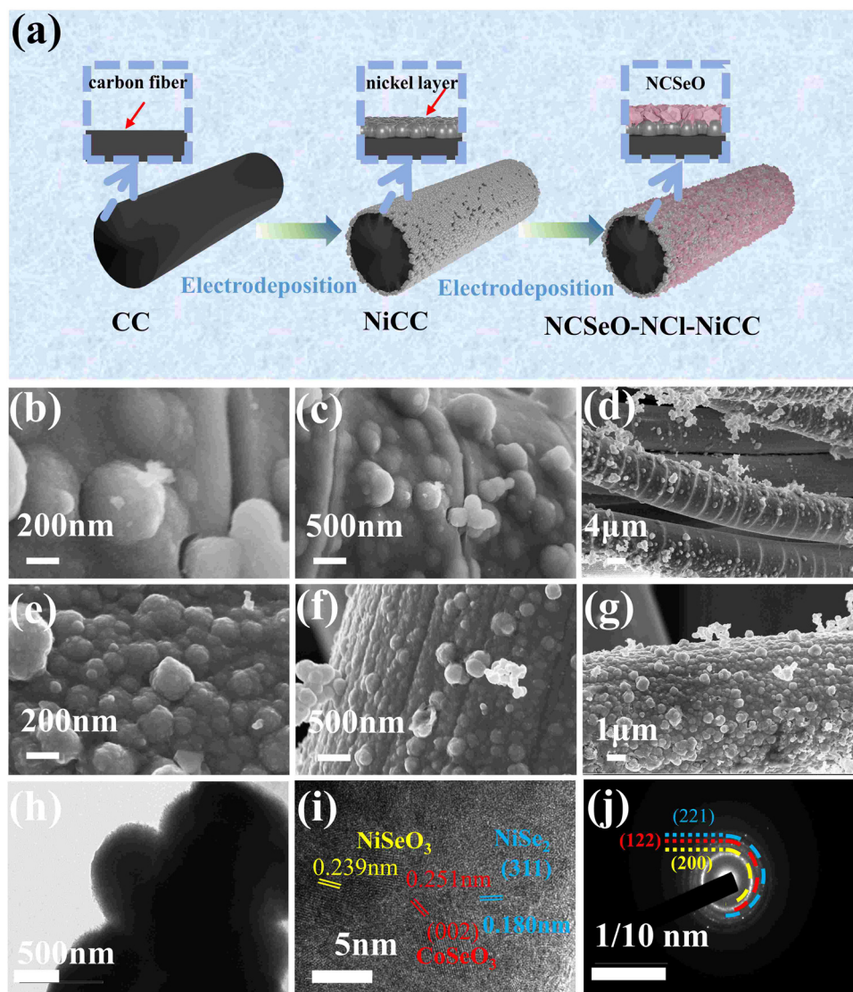
Fig. 1 (a) Schematic of the synthesis process for NCSeO–NiCl–NiCC. (b)–(d) SEM images of NCSeO–Cl–NiCC (e)–(g) SEM images of NCSeO–NiCl–NiCC (h)–(j) TEM, HRTEM and the corresponding SAED images of NCSeO–NiCl–NiCC.
