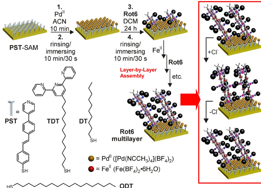
Fig. 8 Layer-by-layer (LbL) nanoarchitectonics of chemically switchable single and multilayers of rotaxanes in a regular pattern on gold surfaces with well-controlled axial shuttling. Reproduced under terms of the CC-BY license from ref. 66, 2015 American Chemical Society.
