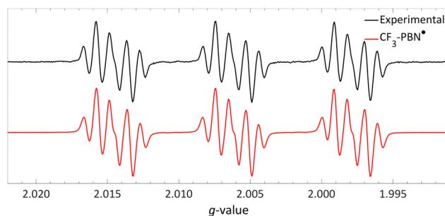
Fig. 17 Room temperature EPR spectrum of the \text{CF}_3 -PBN ^\bullet adduct ( g_{\text{iso}} = 2.0061 , {}^{19}\text{F}a_{\text{iso}} = 0.15 \text{ mT} , {}^{14}\text{N}a_{\text{iso}} = 1.42 \text{ mT} and {}^1\text{H}a_{\text{iso}} = 0.22 \text{ mT} ) after generation due to reduction of the sulfonium salt by NMM in acetonitrile. Further experimental and simulation details are reported in the ESI.†
