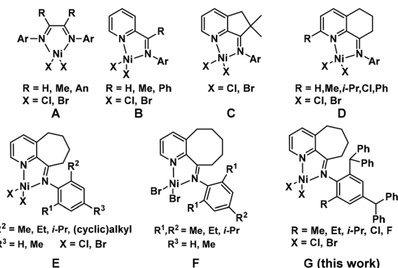
Chart 1 Representative models of N,N -bidentate nickel precatalysts.
