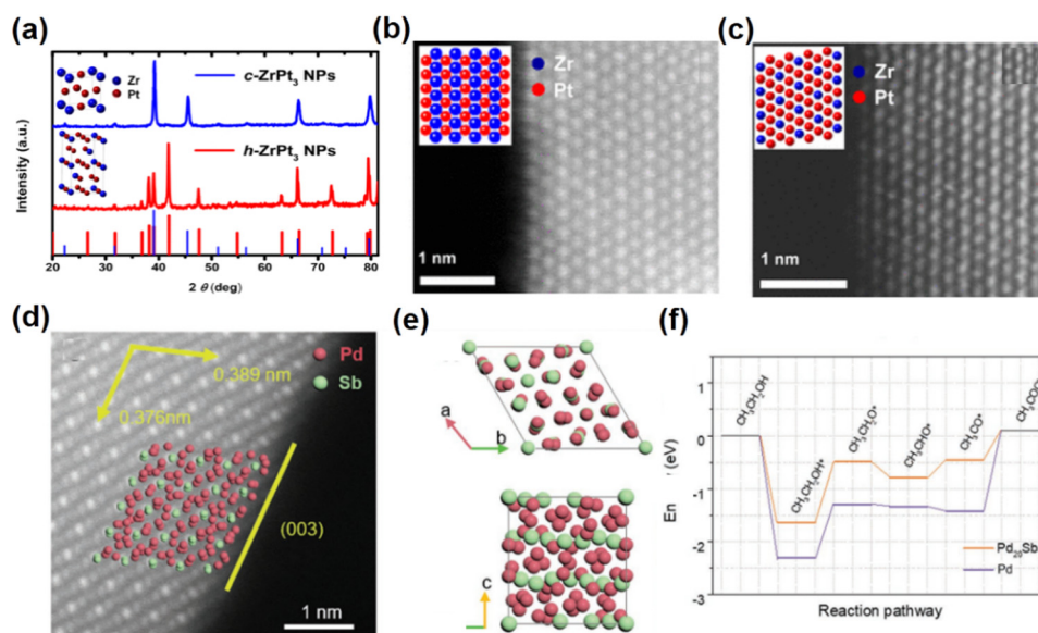
Fig. 5 (a) XRD pattern of the \text{Pt}_3\text{Zr} nanoparticles annealed at 900 °C and 1000 °C. (b) Aberration-corrected HAADF-STEM image of \text{L}_{12}\text{-Pt}_3\text{Zr} . (c) Aberration-corrected HAADF-STEM image of \text{hcp-Pt}_3\text{Zr} . Reproduced with permission from Ref. 57. Copyright 2014, American Chemical Society. (d) Aberration-corrected HAADF-STEM images of \text{Pd}_{20}\text{Sb}_7 rhombohedra. (e) Crystal structure model of \text{Pd}_{20}\text{Sb}_7 . (f) Calculated free energy profiles for the EOR based on \text{Pd}_{20}\text{Sb}_7 and Pd. (d)–(f) Reproduced with permission from Ref. 63. Copyright 2022, John Wiley and Sons.
