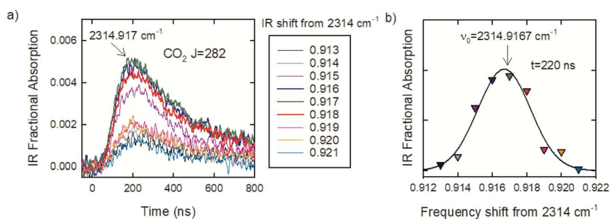
Fig. 3 (a) Transient signals of the \text{CO}_2 R(282) transition collected as a function of IR frequency. (b) The signals at t = 220 \text{ ns} were fit to a Gaussian (black line) to identify the line-center frequency.
