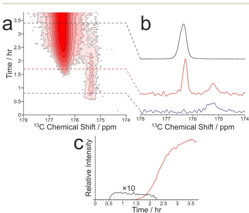
Fig. 3 (a) Intensity contour plot showing the in situ ^1\text{H} \rightarrow ^{13}\text{C} CP NMR spectra recorded as a function of time during crystallization of 1\text{-}^{13}\text{C} -glycine from water–glycerol at -10\text{ }^\circ\text{C} . Contours are based on a log scale with a factor of 2 between adjacent contours. The isotropic peak due to the \beta polymorph is at ca. 175.5 ppm, and the isotropic peak due to the \alpha polymorph is at ca. 176.5 ppm. (b) Selected spectra from (a) recorded at 0.8 h (blue), 1.7 h (red) and 3.4 h (black). (c) Relative intensities of the signals due to the \beta polymorph (black) and \alpha polymorph (red) as a function of time during the crystallization process.
