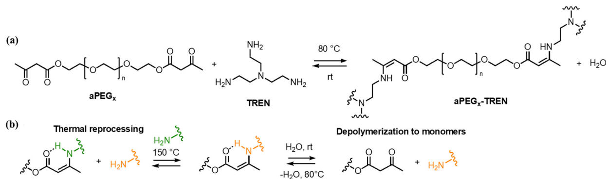
Scheme 7 (a) Synthesis of the vinyllogous urethane network from bis(acetoacetate)-terminated poly(ethylene glycol) (aPEG x ) and tris(2-aminoethyl) amine (TREN) as the crosslinker. (b) Transamination between an amine and a vinyllogous urethane (left) and the reversible hydrolytic depolymerization to the parent monomers (right). Reproduced from ref. 185 with permission from Wiley, copyright 2023.
