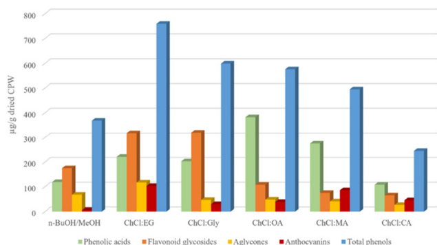
Fig. 4 Distribution of different phenol classes in cherry pomace waste (CPW) extracts ( \mu\text{g g}^{-1} of dried CPW) obtained using classical solvents and (NA)DESSs.
